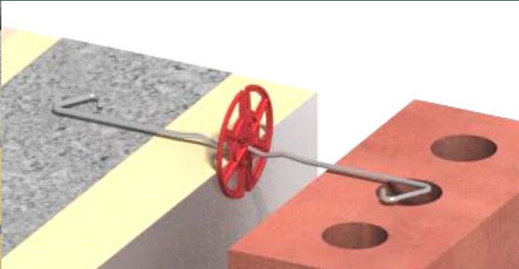
PLASTIC INSULATION DISCS
